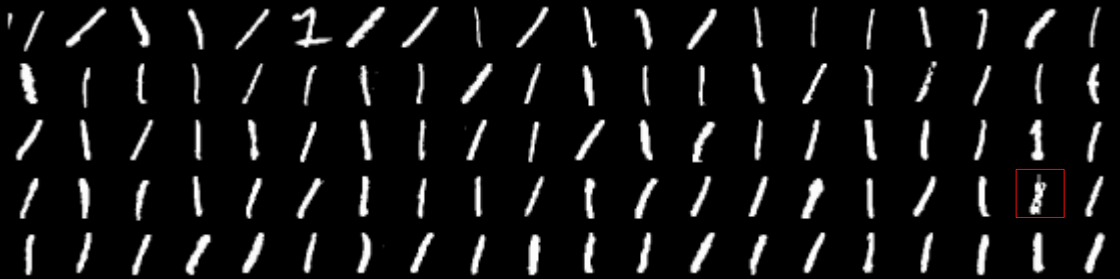
One-Class SVM
